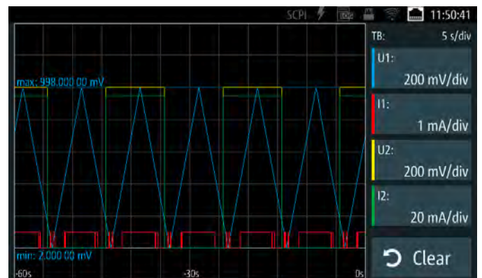
Graphical View on an R&S®NGP800.
